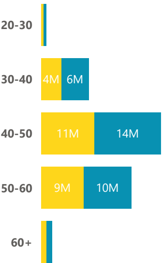
Age Group
