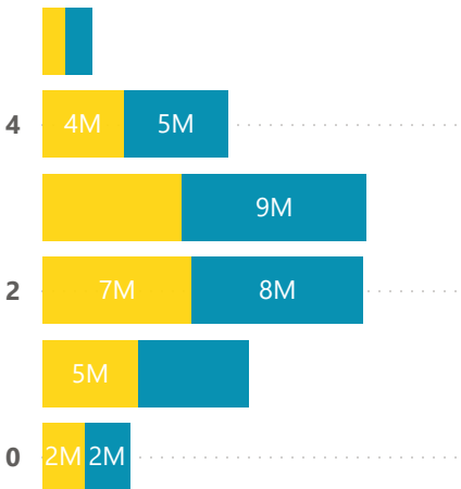
Dependent Count
